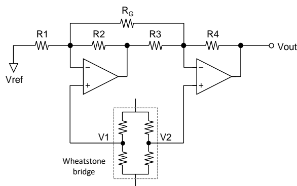
Figure 16. Bridge Amplifier
