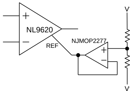
Fig.5. Example of a low impedance reference circuit.
