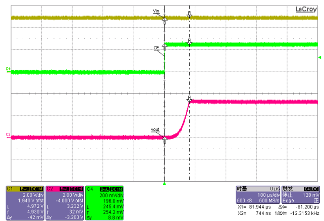
CE Chip Enable Response
