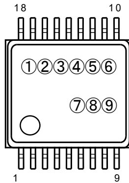
HSOP-18 Part Markings
