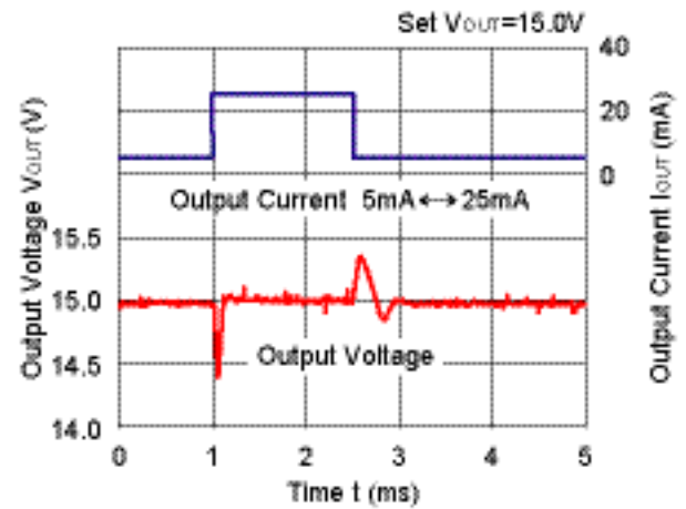
18) Load Transient Response (V IN =3.6V, I OUT =5mA↔25mA, t r =t f =0.5μs)
